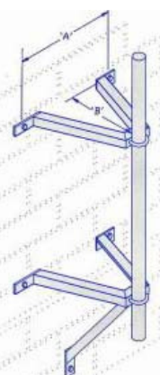
Stand-Off Bracket
